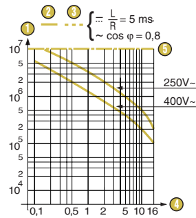
Operating curve for type 831600
