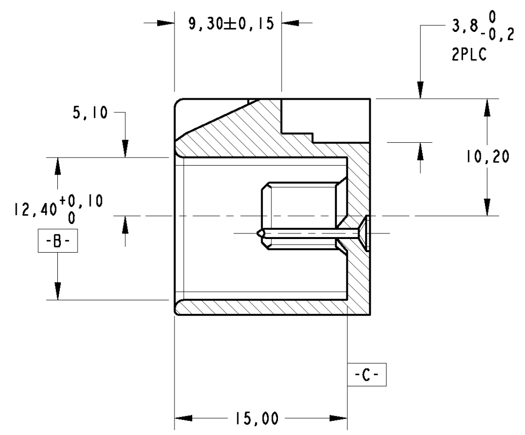
SECTION B-B
