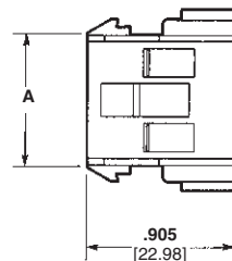
Cap Front
