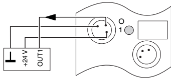
Connection diagram
