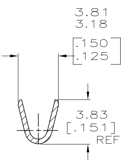
SECTION B-B
