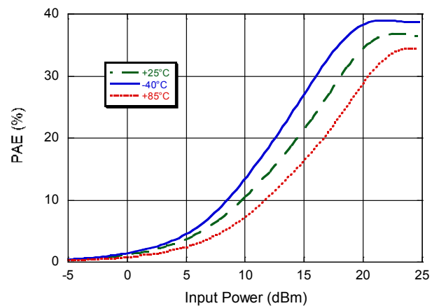
Power Added Efficiency vs. Input Power @ 5.6 GHz
