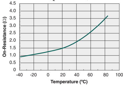
Typical On-Resistance vs. Temperature ( I_L = \text{Max Rated} )
