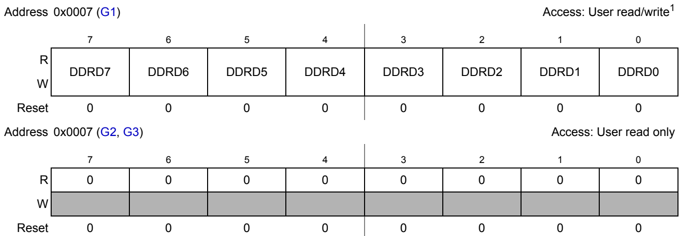
Figure 2-9. Port D Data Direction Register (DDR)
