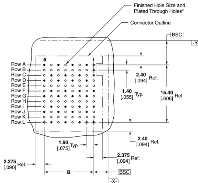
* Finished Hole Diameter = 0.46 \pm^{0.05}_{0.018 \pm^{0.002}} Drilled Hole Diameter = 0.55 \pm^{0.02}_{0.022 \pm^{0.001}} Copper Thickness = 0.038 \pm^{0.013}_{0.0015 \pm^{0.0005}} Tin-Lead Thickness = 0.008 \pm^{0.004}_{0.0003 \pm^{0.0002}} Finishes other than Tin-Lead. See Appl. Spec. 114-13202
