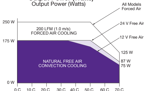
Figure 1: Derating Curve Output Power (Watts) Output Power (Watts)
