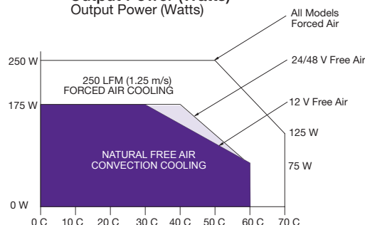
Figure 1b: Derating Curve With Cover Output Power (Watts) Output Power (Watts)
