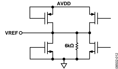
Figure 57. Equivalent VREF Circuit
