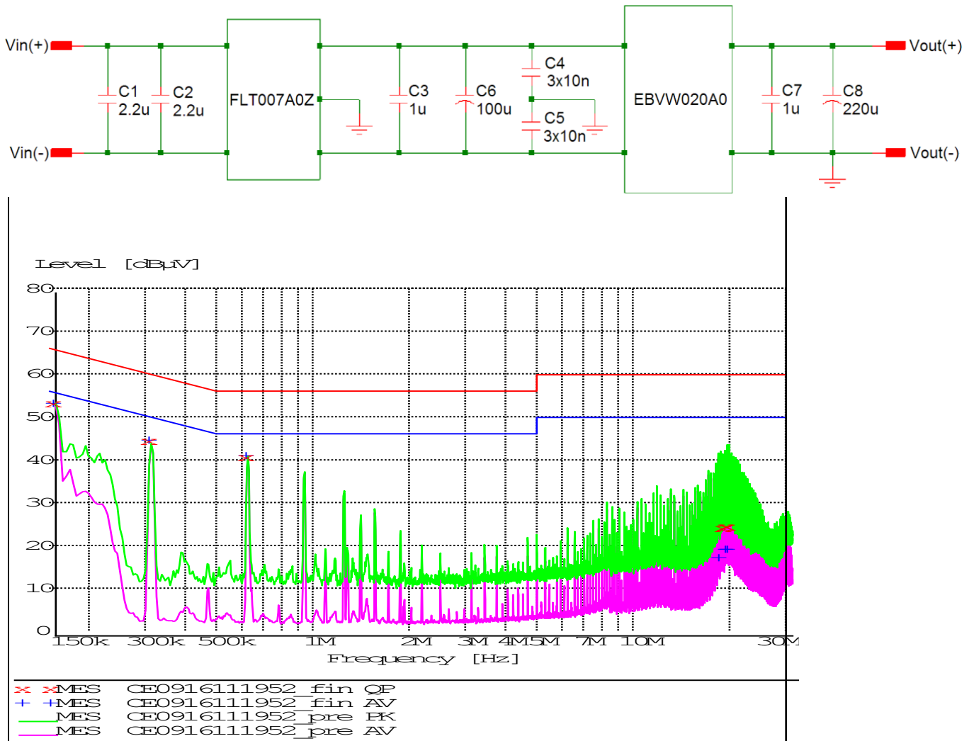
Figure 24. EMC Considerations.
