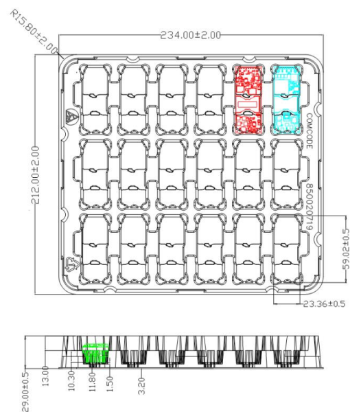
Base Plate Module Tray
