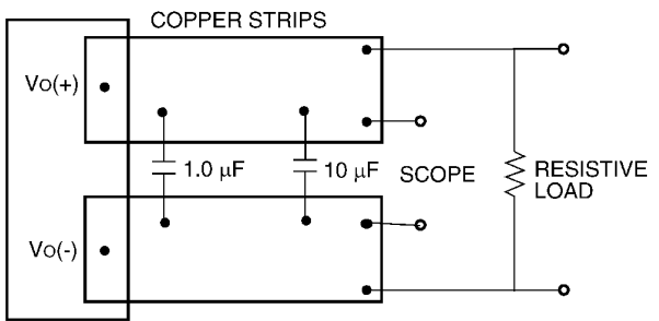
Figure 12. Input Reflected Ripple Current Test Setup.
