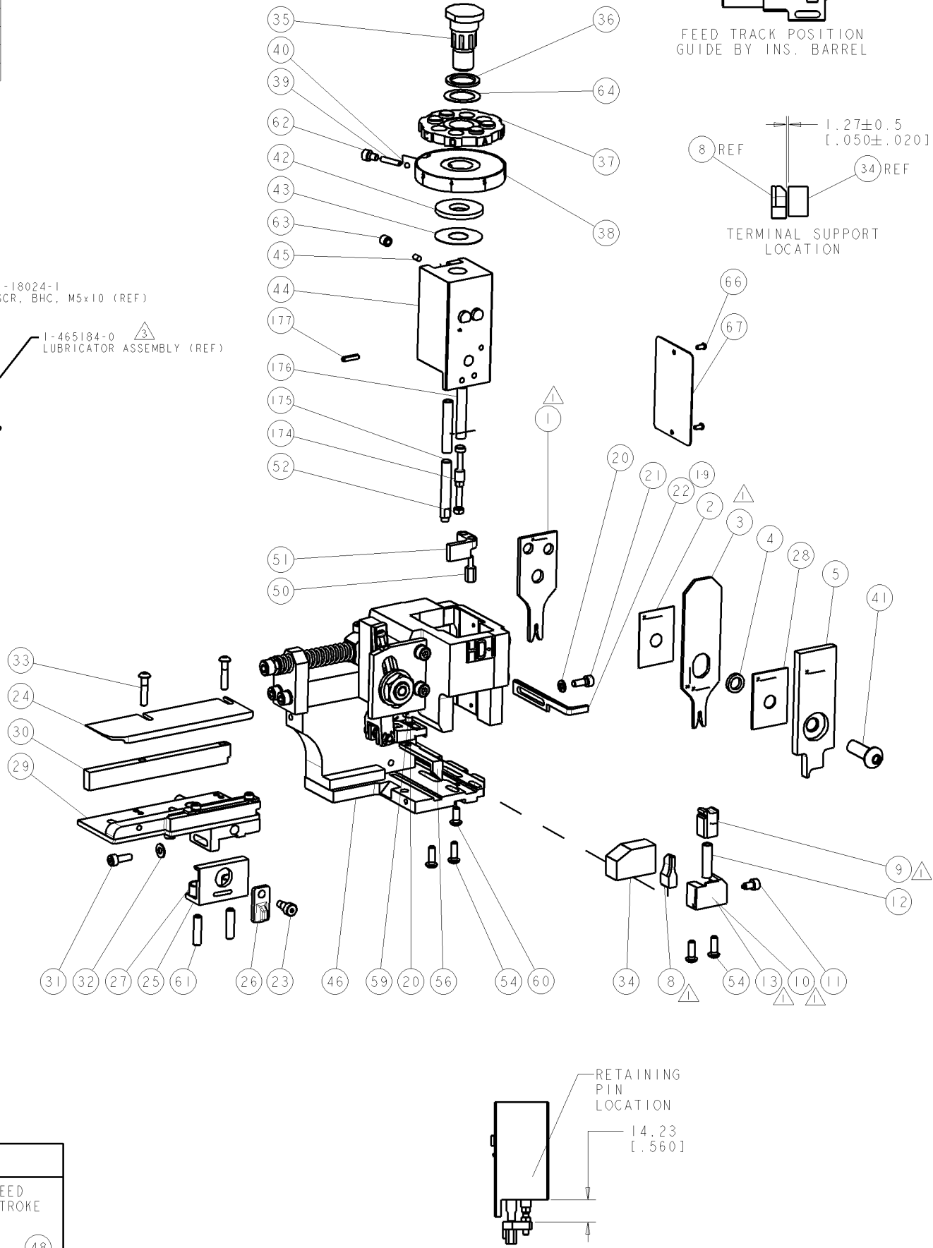
HOLDDOWN SET-UP
