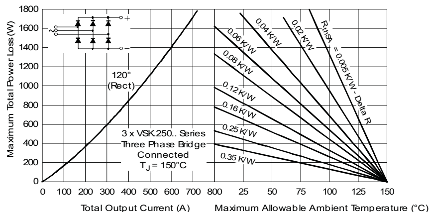
Fig. 7 - Forward Power Loss Characteristics
