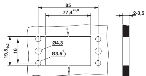
Mounting cutout
