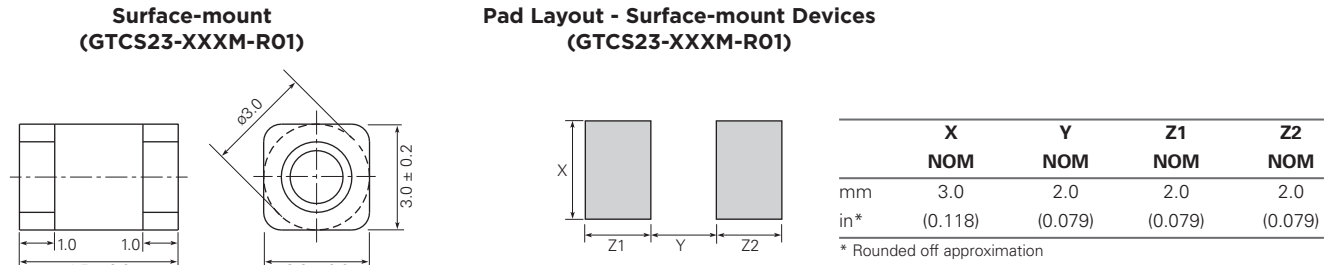
Figure G4 Two Electrode 5mm Product Dimensions
