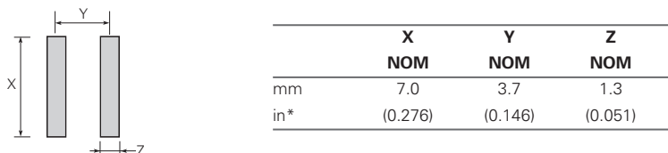
Pad Layout - Surface-mount Devices (GTCS26-XXXM-R05)
