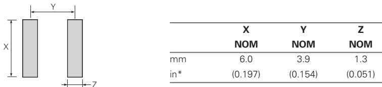
Pad Layout - Surface-mount Devices (GTCS25-XXXM-R02)
