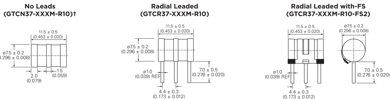
Figure G9 Three Electrode 7mm Product Dimensions
