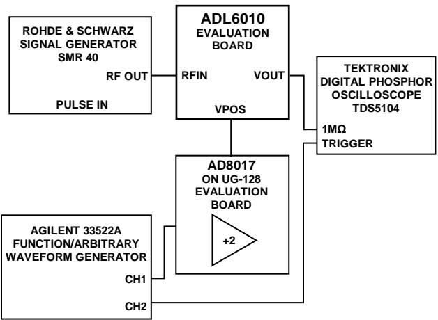
Figure 35. Hardware Configuration for Output Response to Power Supply Gating Measurements
