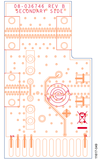
Figure 46. ADL6010 Evaluation Board Layout, Bottom Side
