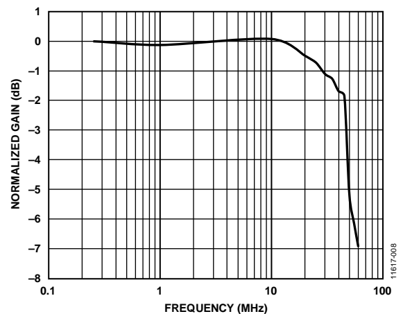
Figure 7. Envelope Bandwidth of V_{OUT} vs. Frequency at P_{IN} = -10 dBm and Modulation Depth = 10% (See Figure 36 in the Measurement Setups Section)
