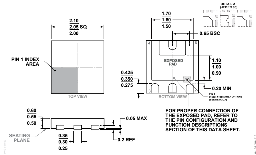
Figure 47. 6-Lead Lead Frame Chip Scale Package [LFCSP] 2.05 mm x 2.05 mm Body and 0.55 mm Package Height (CP-6-7) Dimensions shown in millimeters
