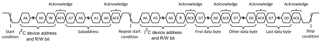
Figure 34. Multiple-Byte Read Transfer
