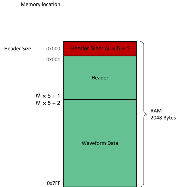
Figure 25. RAM Structure
