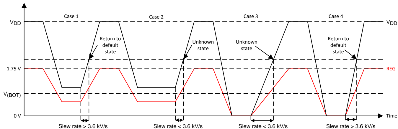
Figure 22. Brownout Behavior
