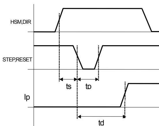
Fig.4 Timing chart
