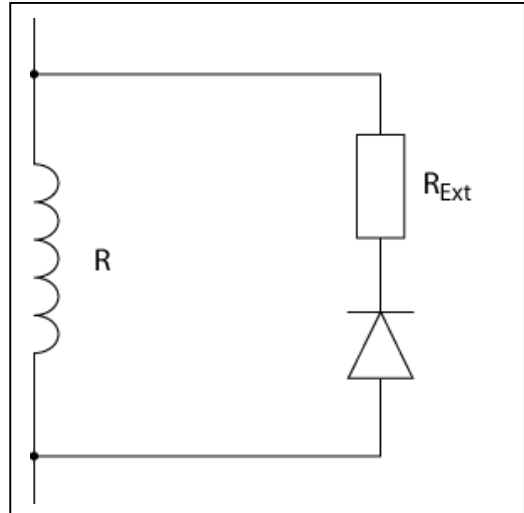
Fig. 12 Resistor and turn off circuit
