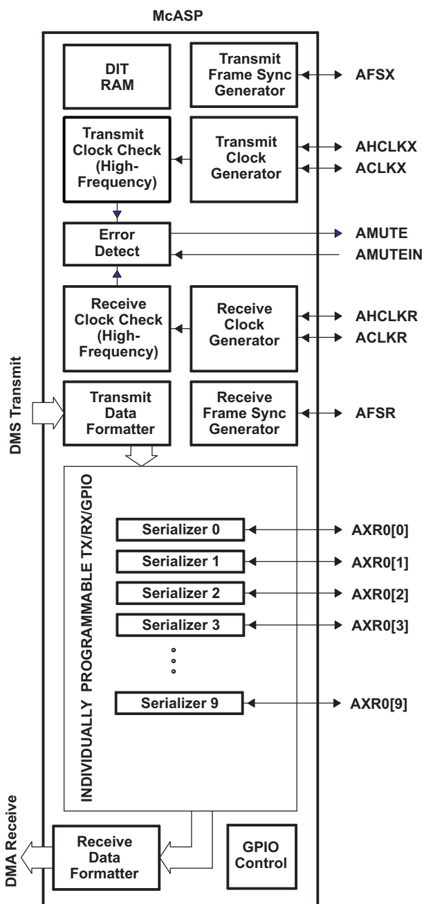
Figure 6-42. McASP Configuration
