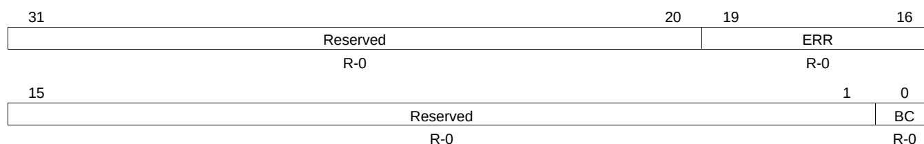
Figure 3-3. BOOTCMPLT Register 3
