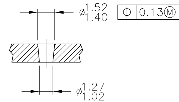
SECTION A-A SCALE 5:1
