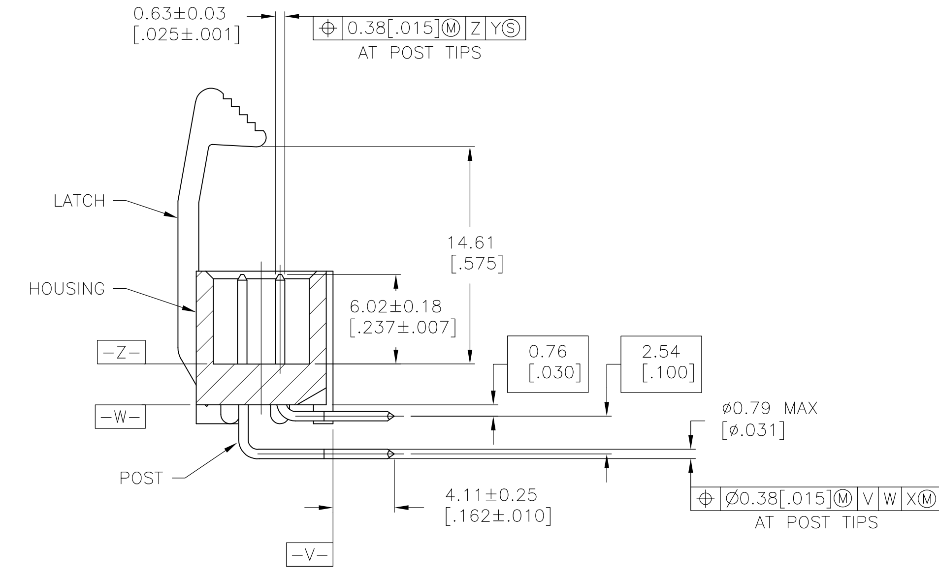
SECTION U-U
