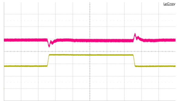
Fig. 12: Output voltage response to load current step change (36 A – 54A – 36 A) at V_{in} = 48 V. Top trace: output voltage (500 mV/div.). Bottom trace: load current (20 A/div.). Current slew rate: 1 A/ \mu s. C_o = 1 \mu F ceramic + 10,000 \mu F tantalum. Time scale: 200 \mu s/div.
