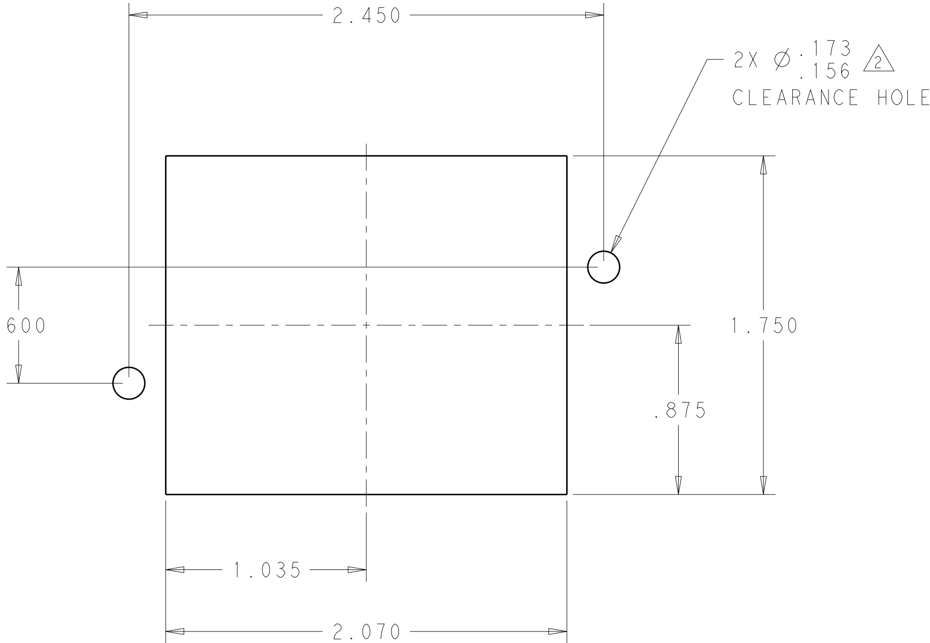
PIN CONNECTOR PANEL CUT-OUT
