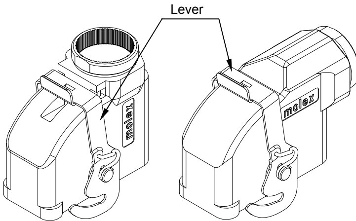
58696-0010 (Straight type)
