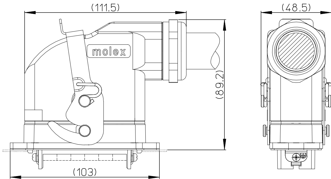
Right-angle type
