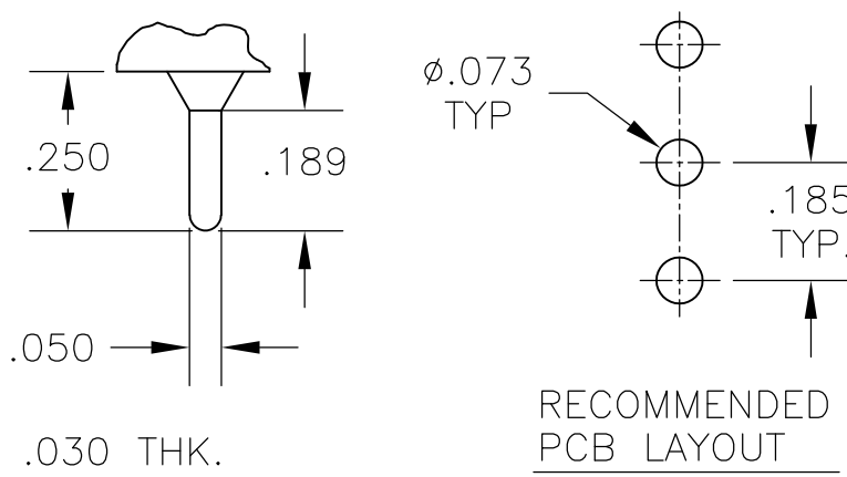
C PRINTED CIRCUIT
