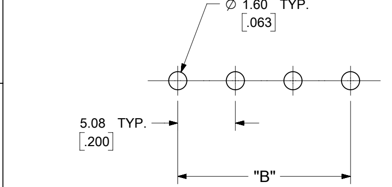
PCB LAYOUT
