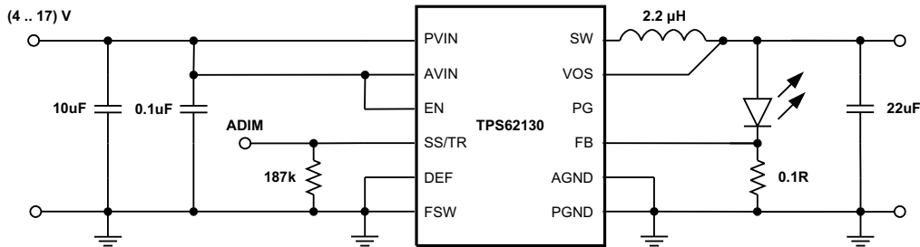
Figure 46. Single Power LED Supply
