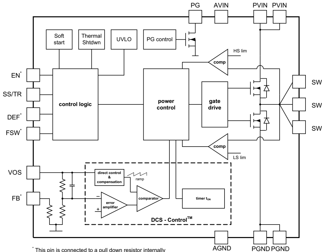
Figure 6. TPS62131/2/3 (Fixed Output Voltage)
