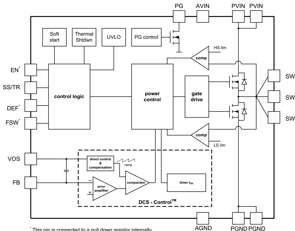
Figure 5. TPS62130 and TPS62130A (Adjustable Output Voltage)
