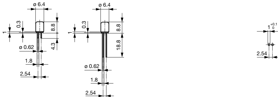
Drilling diagram
