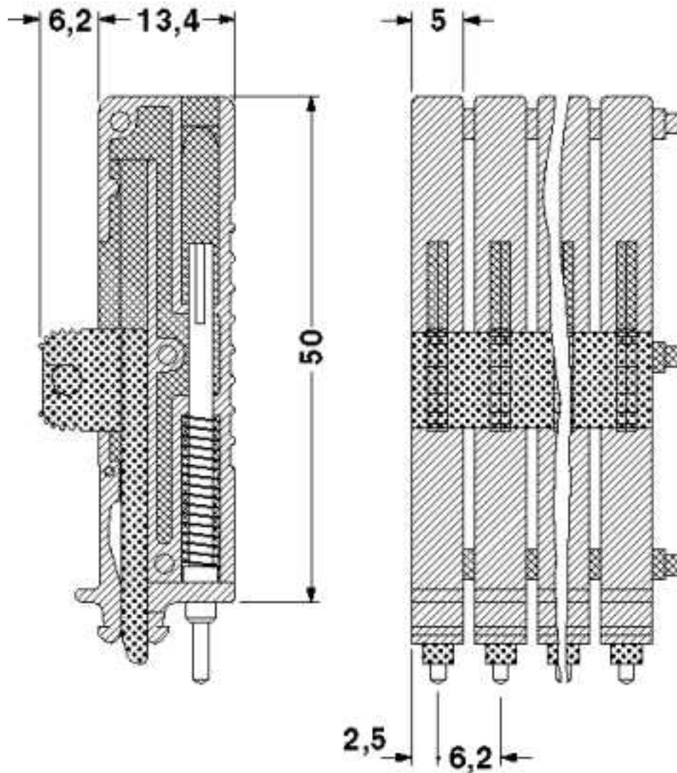
Dimensional drawing
