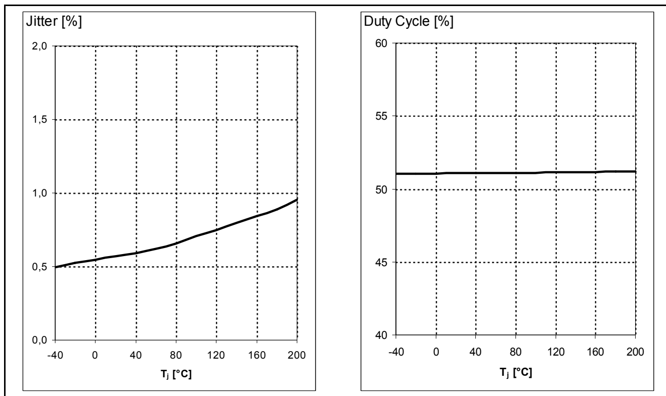
Figure 16 Jitter 1\sigma at \Delta B = 2 mT at 1 kHz (left), Duty Cycle [%] \Delta B = 2 mT at 1 kHz (right)
