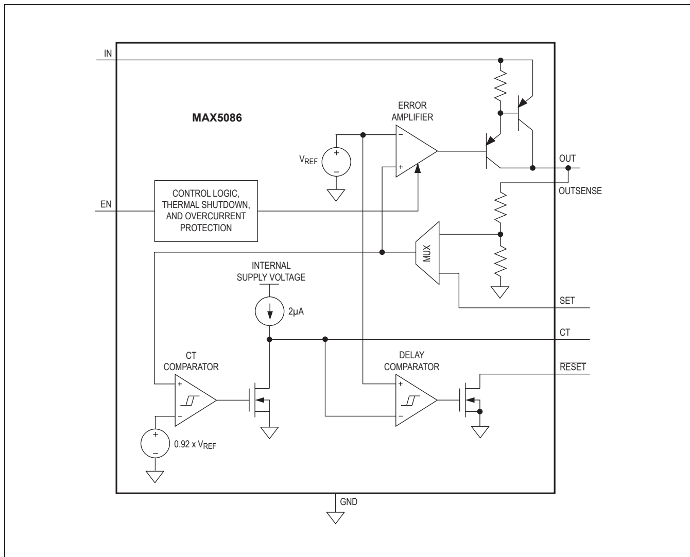
Figure 1. Functional Diagram
