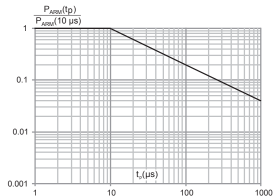
Figure 4. Normalized avalanche power derating versus pulse duration ( T_j = 125^\circ\text{C} )
