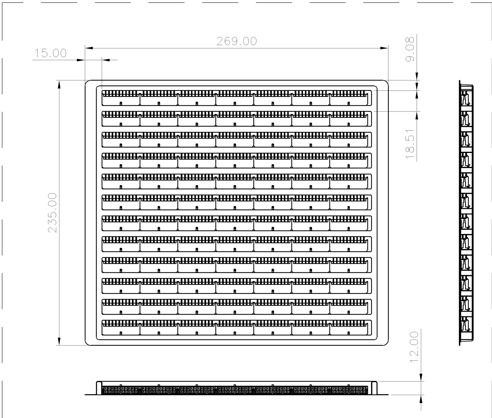
TRAY DETAIL
