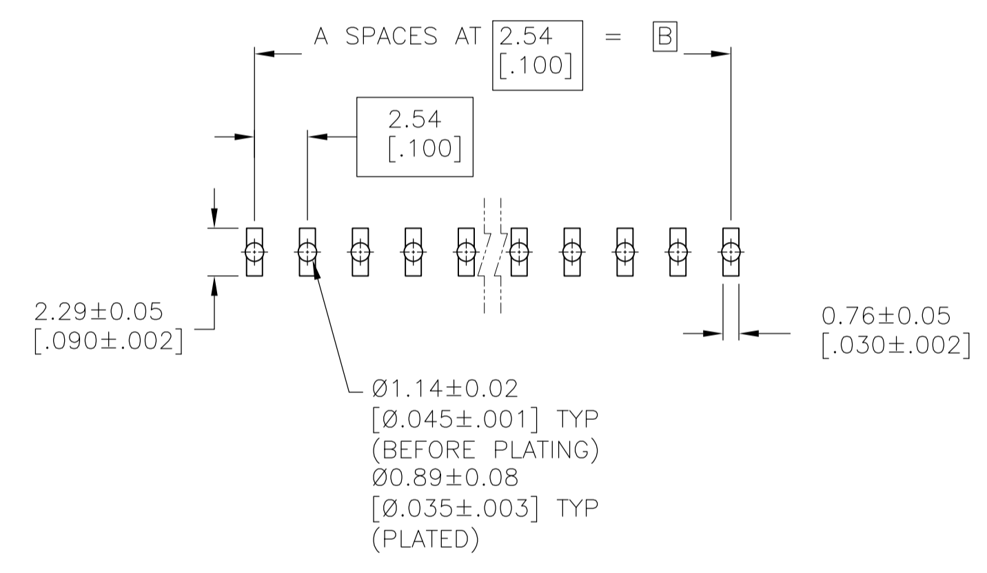
RECOMMENDED PC BOARD MOUNTING DIMENSIONS FOR .063 [1.60] THICK PC BOARD AND .012 [3.05] STENCIL THICK.
