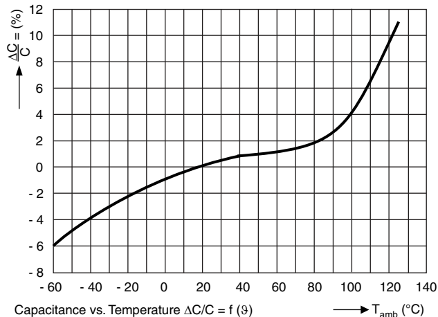
Capacitance vs. Temperature \Delta C/C = f(\theta) Capacitance as a function of temperature \Delta C/C = f(T_A), T_{LL} \leq T_A \leq T_{UL}
