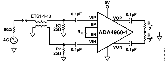
Figure 31. Differential-Input-to-Differential-Output Configuration
