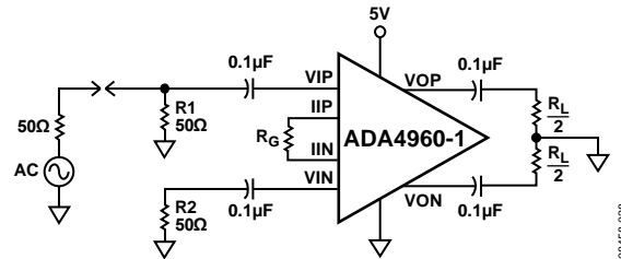
Figure 32. Single-Ended-Input-to-Differential-Output Configuration
