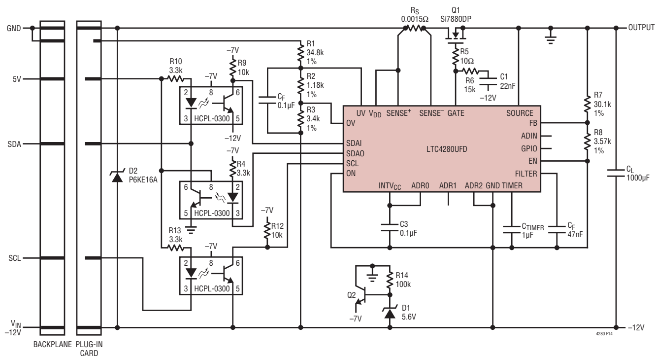
-12V Card Resident Application with Optically Isolated I 2 C and a 16.6A Circuit Breaker
