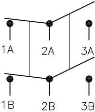
SWITCH FUNCTION D1 CIRCUIT DIAGRAM
