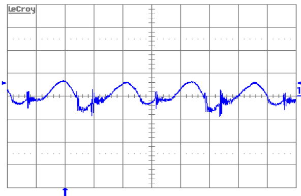
Figure 10. Output voltage ripple (20 mV/div.) at full rated load current into a resistive load with C_o = 10\mu\text{F tantalum} + 1\mu\text{F} slew rate: 5A/ \mu\text{s} . C_o = 470\mu\text{F POS} + 1\mu\text{F cer. ceramic} and V_{in} = 48\text{ V} . Time scale: 1 \mu\text{s}/\text{div} . Time scale: 0.2ms/div.
