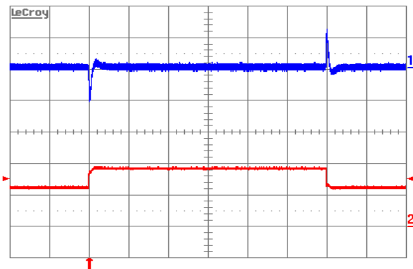
Figure 9. Output voltage response to load current step-change (12.5A–18.75A–12.5A) at V_{in} = 48\text{ V} . Top trace: output voltage (100 mV/div.). Bottom trace: load current (10A/div.). Current
