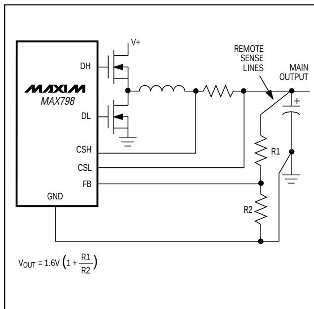
Figure 5. Adjusting the Output Voltage
