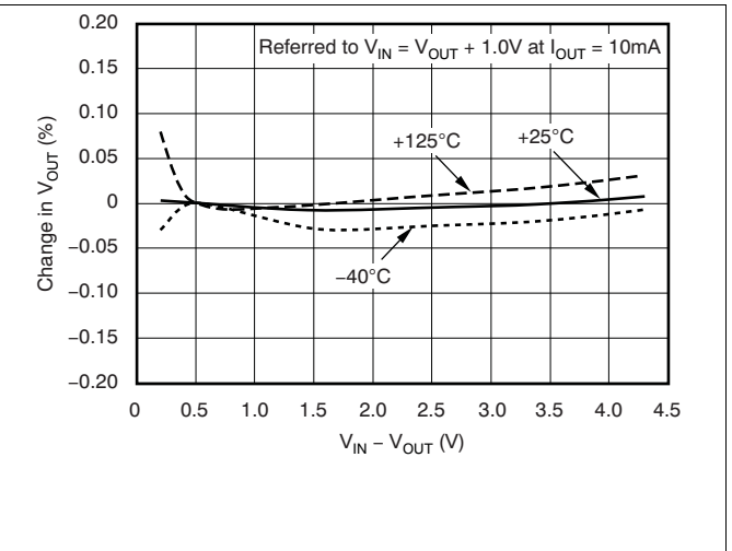
Figure 2. Line Regulation
