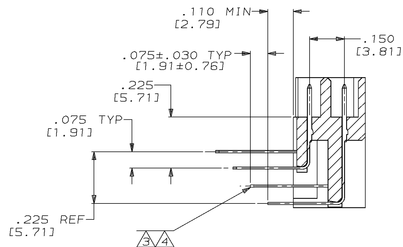
SECTION X-X
