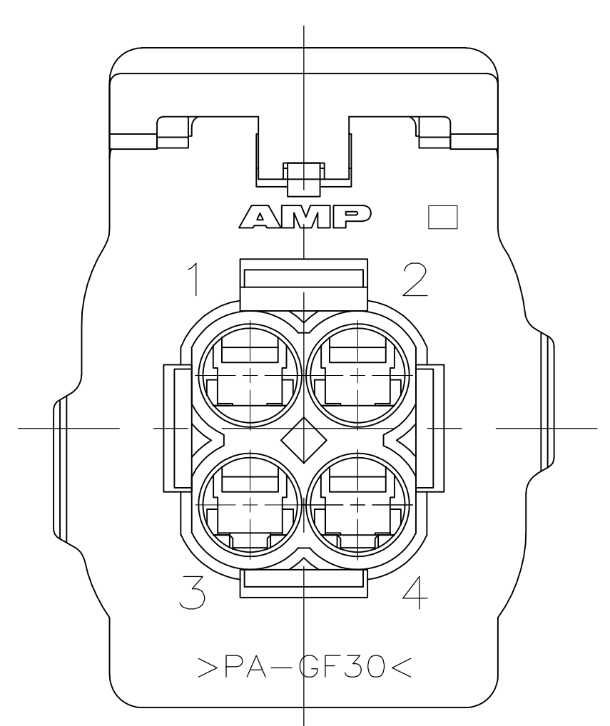
VIEW B-B
