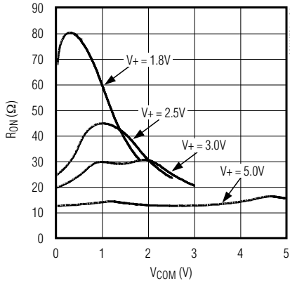
ON-RESISTANCE vs. V_{\text{COM}}
