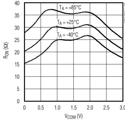
ON-RESISTANCE vs. V_{\text{COM}} ( V_+ = 3\text{V} )
