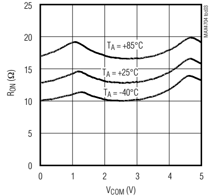
ON-RESISTANCE vs. V_{\text{COM}} ( V_+ = 5\text{V} )
