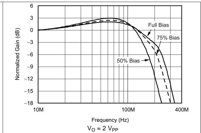
Figure 44. Small-Signal Frequency Response vs Bias
