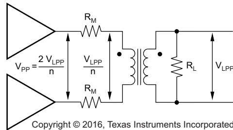
Figure 85. Driver Peak Output Voltage
