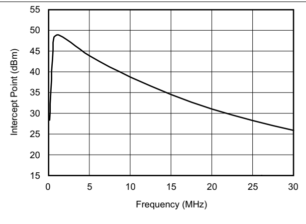
Figure 42. Two-Tone, Third-Order Intermodulation Intercept
