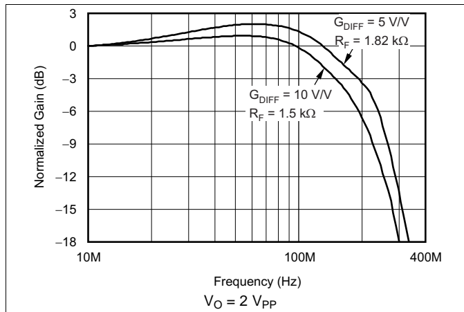
Figure 43. Small-Signal Frequency Response
