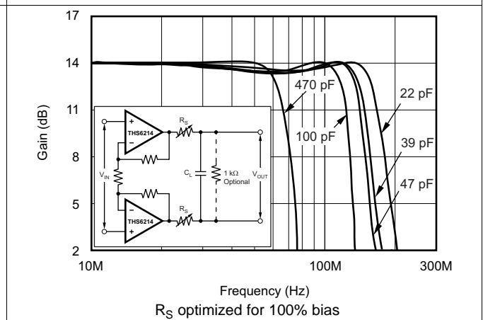
Figure 48. Frequency Response vs Capacitive Load
