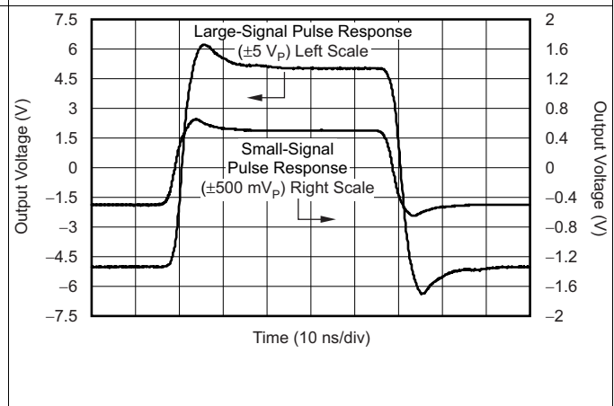
Figure 46. Pulse Response
