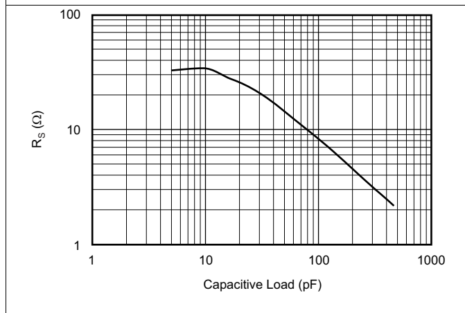
Figure 47. Recommended R_S vs Capacitive Load
