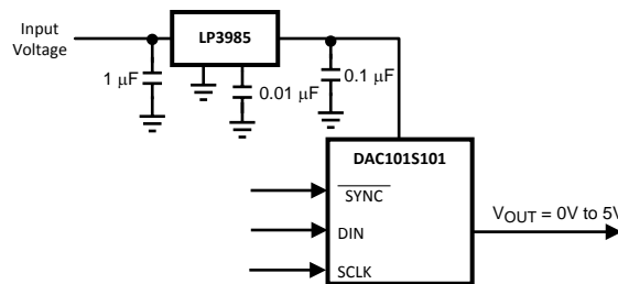
Figure 45. Using The Lp3985 Regulator
