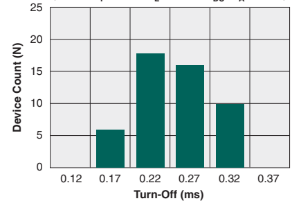
Typical Turn-Off Time (N=50, I F =5mA, I L =100mA DC , T A =25°C)
