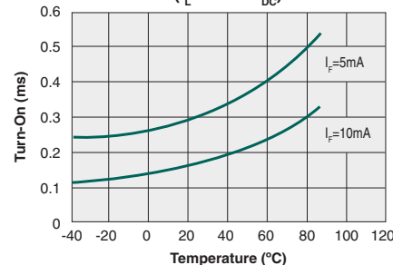
Typical Turn-On vs. Temperature (I L =100mA DC )
