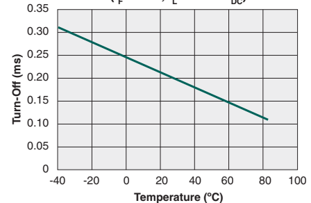
Typical Turn-Off vs. Temperature (I F =5mA, I L =100mA DC )
