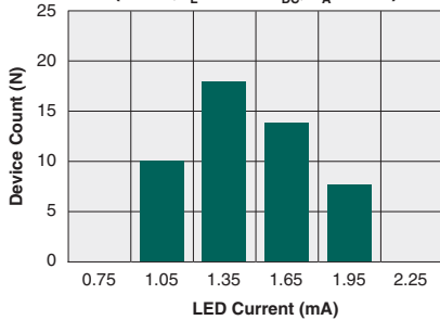
Typical I F for Switch Operation (N=50, I L =100mA DC , T A =25°C)
