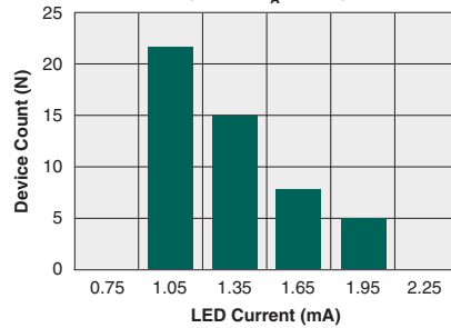
Typical I F for Switch Dropout (N=50, T A =25°C)
