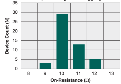
Typical On-Resistance Distribution (N=50, I F =5mA, I L =100mA DC , T A =25°C)
