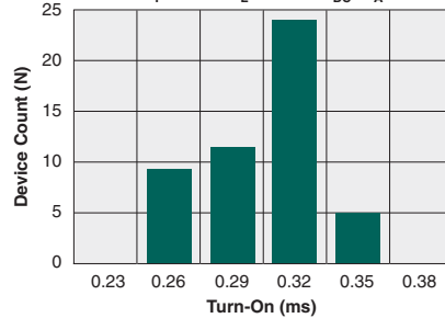
Typical Turn-On Time (N=50, I F =5mA, I L =100mA DC , T A =25°C)
