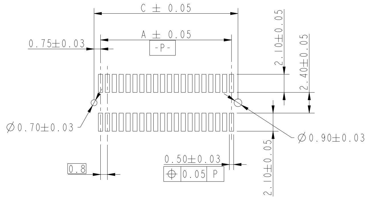
RECOMMENDED PCB LAYOUT WITH PLASTIC PEG
