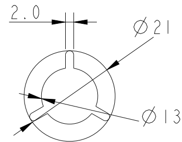
DETAIL H
