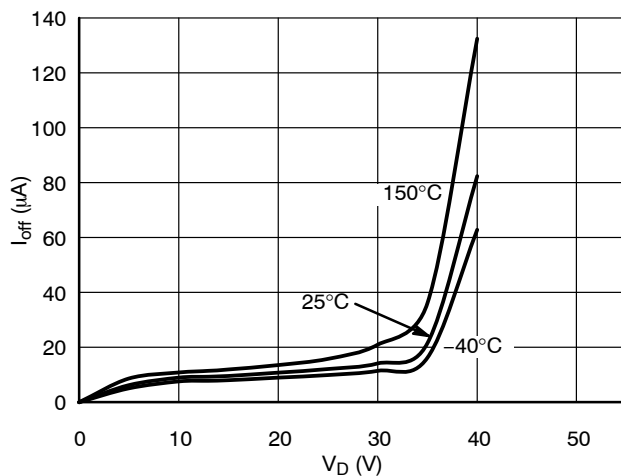
Figure 8. OFF State Standby Current vs. V D
